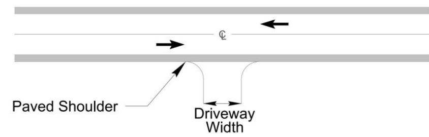
Figure 4-9 Driveways Tying to Paved Shoulders
