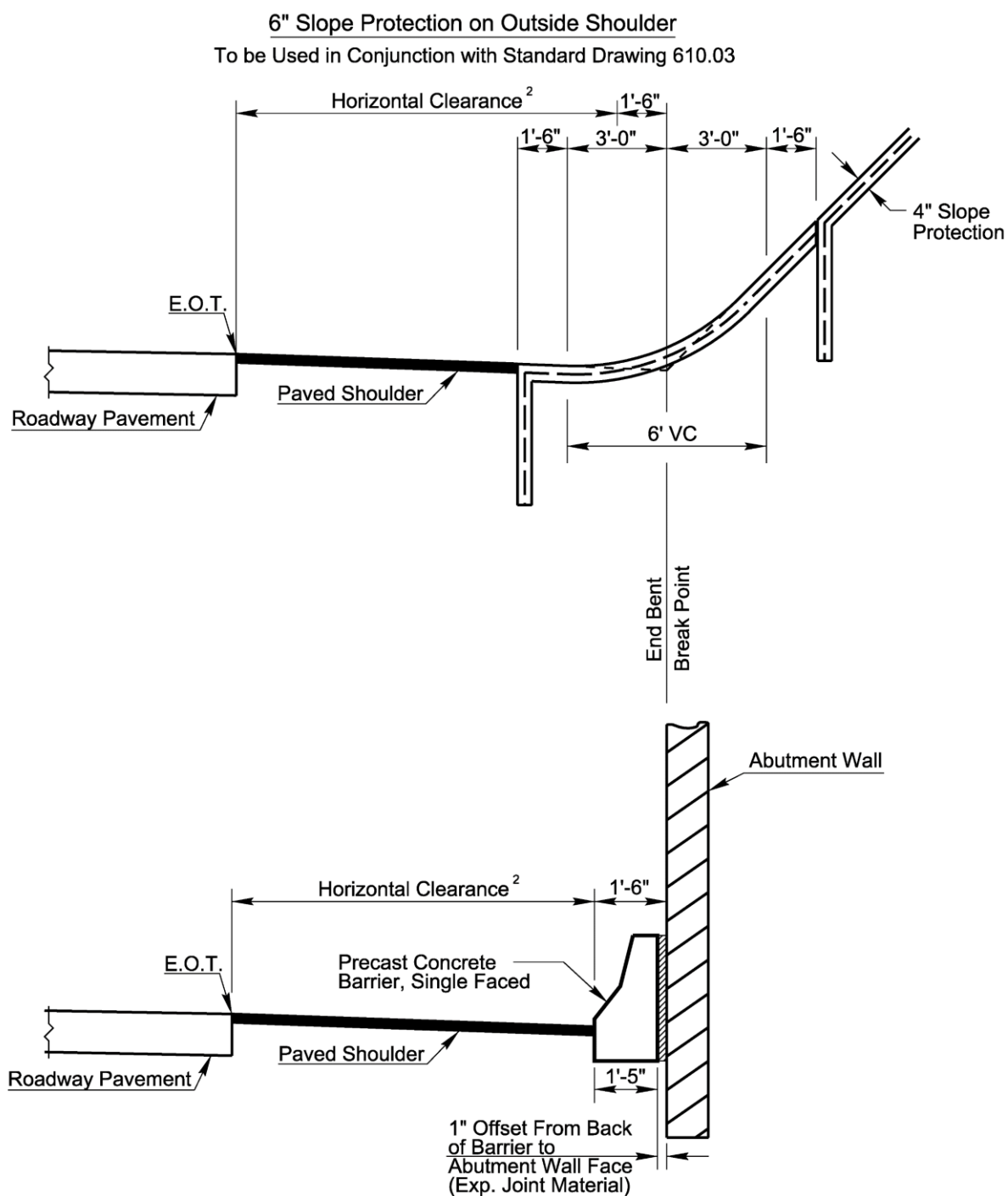
Figure 5-21 Shoulder Detail Under Bridge with 6-Inch Slope Protection or Abutment Wall
