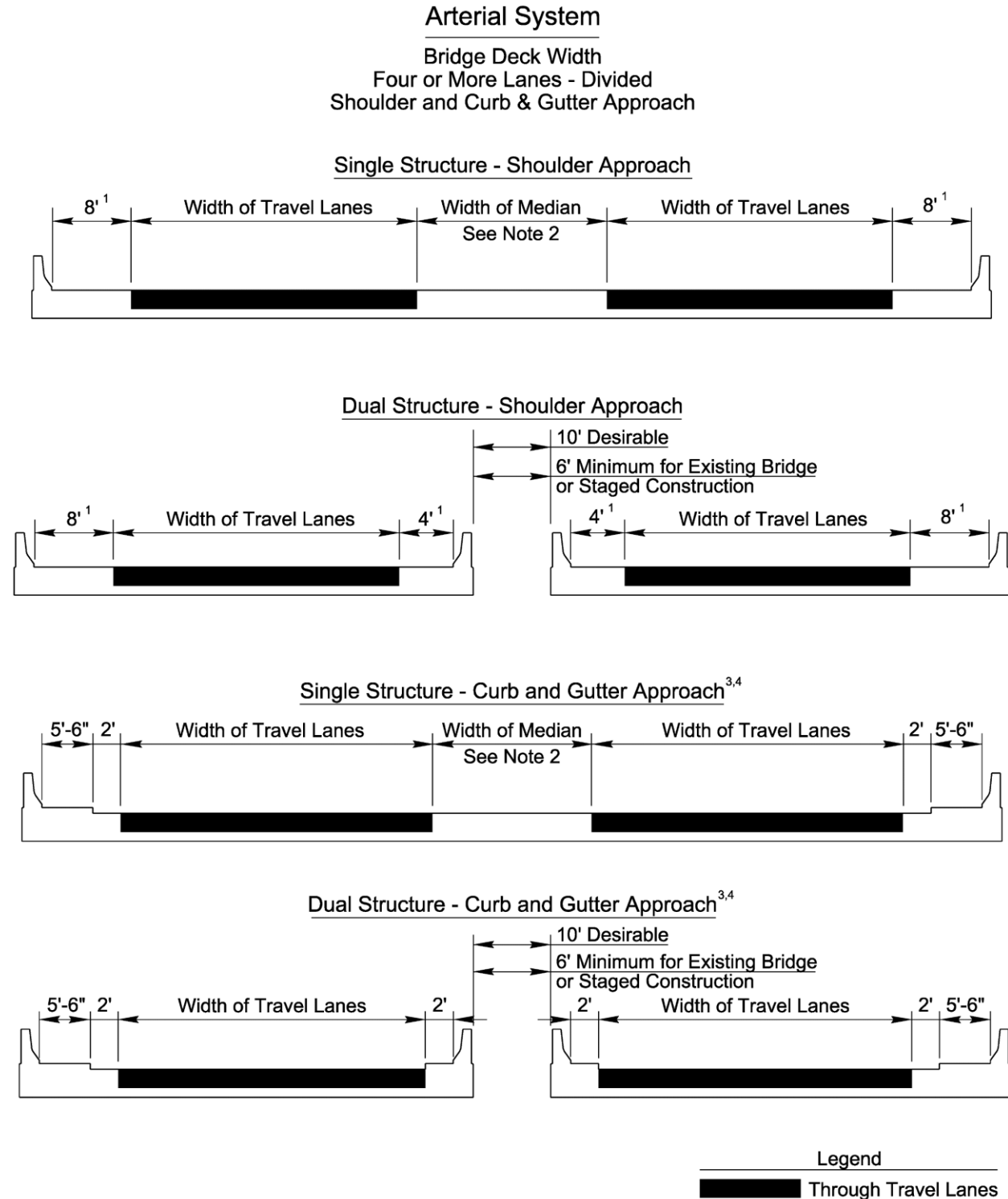
Figure 5-4 Arterial System Bridge Deck Widths for Four or More Lanes Divided Shoulder Approach and Curb and Gutter Approach
