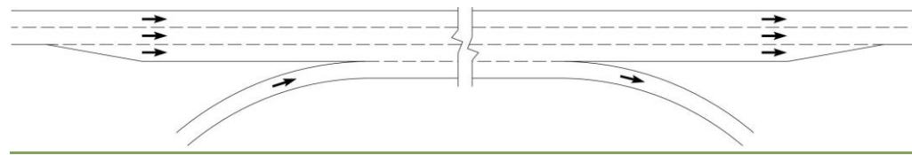
Figure 9-2 Adding Auxiliary Lanes for Improved Weaving Operations
